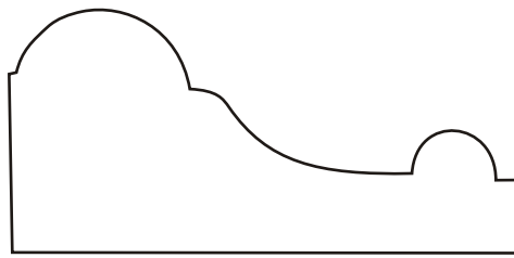
CR-7 1-1/8 x 2-1/2 CHAIR RAIL
